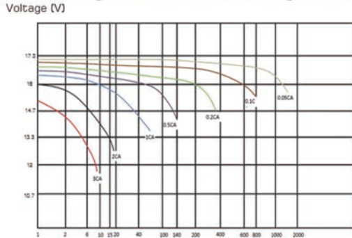
Discharge Curves at Different Discharge Rate (25°C)
