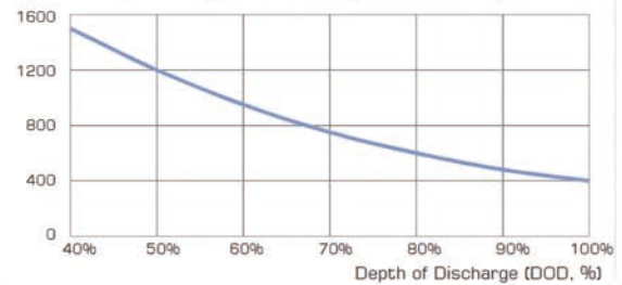
Cycle Life (Cycles) Cycle Life vs. Depth of Discharge
